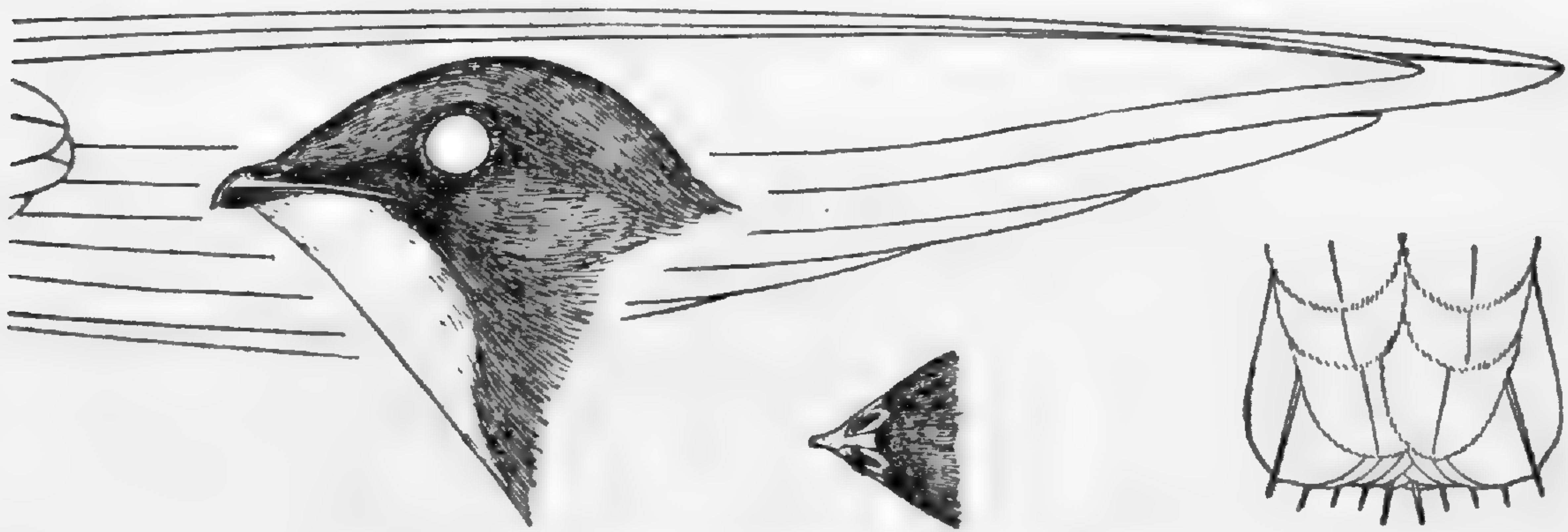
FIG. 3. Chætura picina Tweeddale; generic details, X 1.
